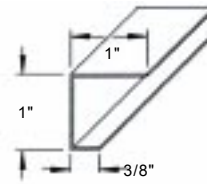
1" Channel C
