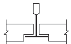
TEGULAR
