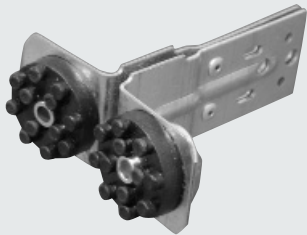
RSIC-DC04X2™ Clip
