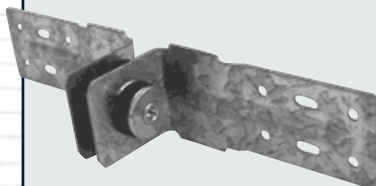
RSIC-CWB™ Clip
