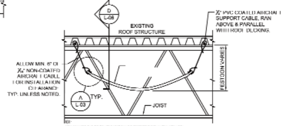
4 PANEL - TYP. CABLE END ATTACHMENT DETAIL SCALE: NA
