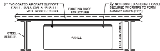
E HORZ. LANYARD - CABLE END ATTACHMENT DETAIL SCALE: NA
