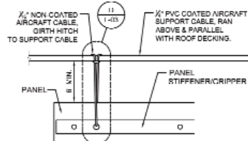
A PANEL - TYP. CABLE END ATTACHMENT DETAIL SCALE: NA
