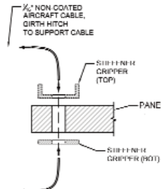
D HARDWARE ATTACHMENT DETAIL SCALE: NA
