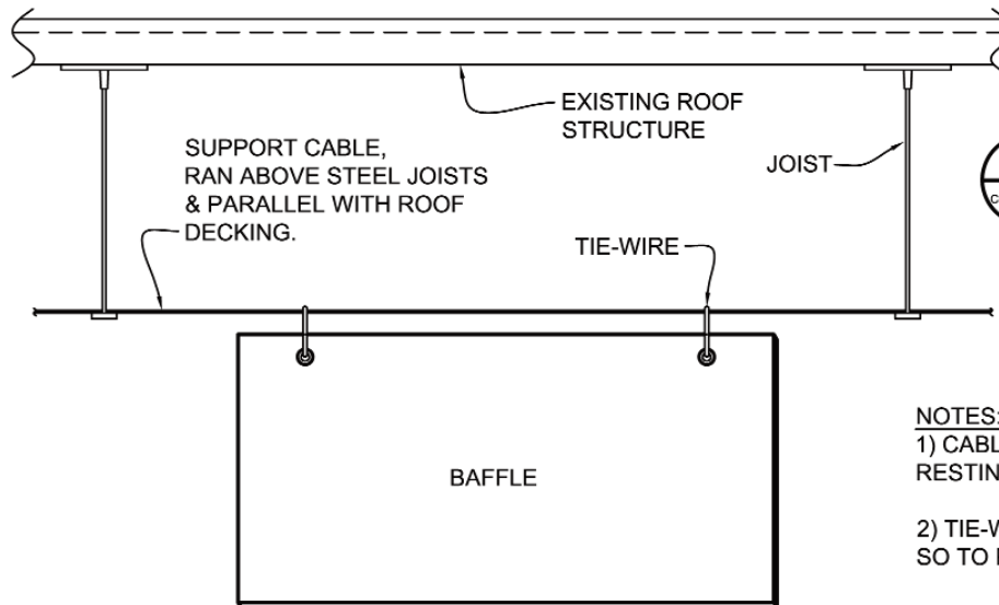
FRONT ELEVATION
