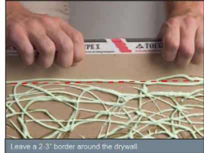
Leave a 2-3" border around the drywall
