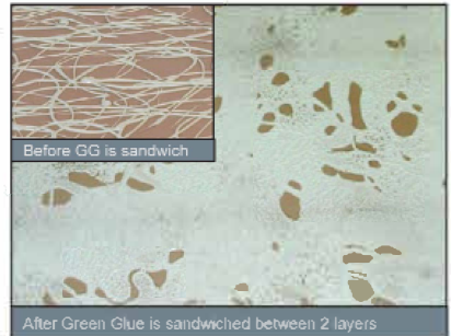
After Green Glue is sandwiched between 2 layers
