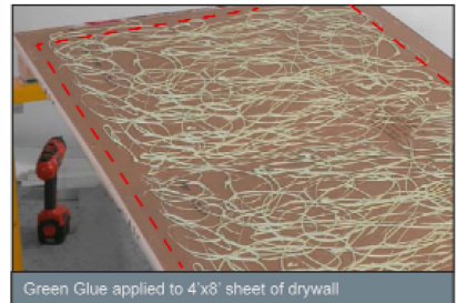
Green Glue applied to 4x8 sheet of drywall
