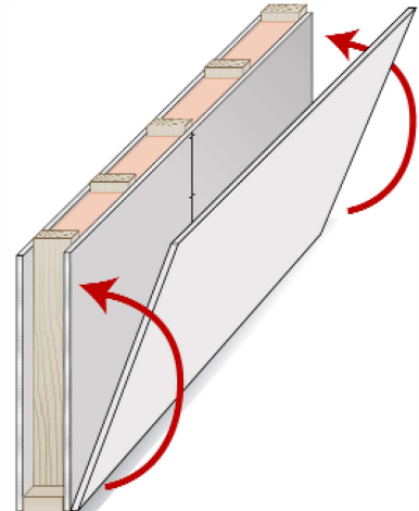
After Green Glue is sandwiched between 2 layers
