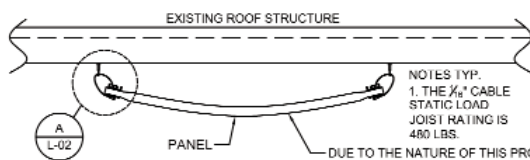
2 L-02 PANEL - TYP. END ATTACHEMENT DETAIL SCALE: NA
