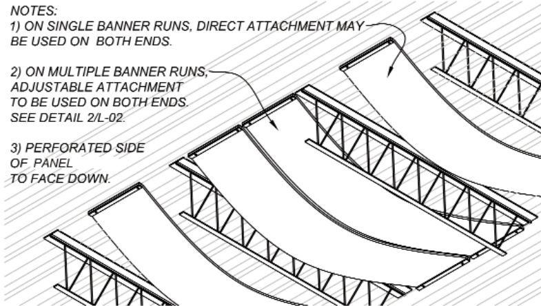
1 L-02 VIEW FROM BELOW SCALE: NA
