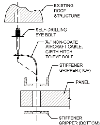
A L-02 HARDWARE ATTACHMENT DETAIL SCALE: NA
