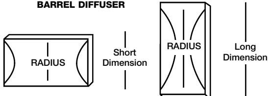
BARREL DIFFUSER
