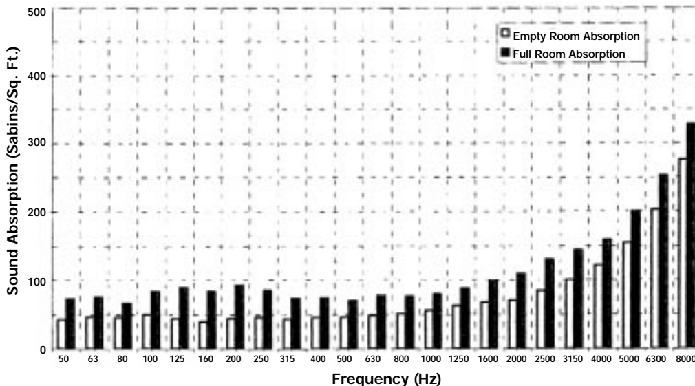
Sound Absorption - Empty vs. Full
